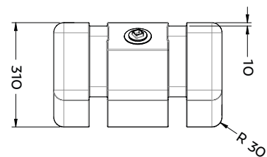
Base View
