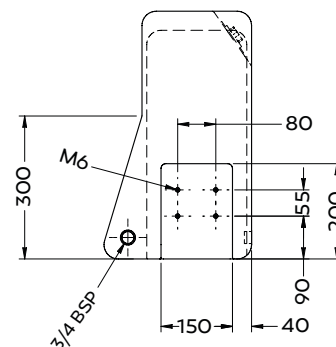
Base View
